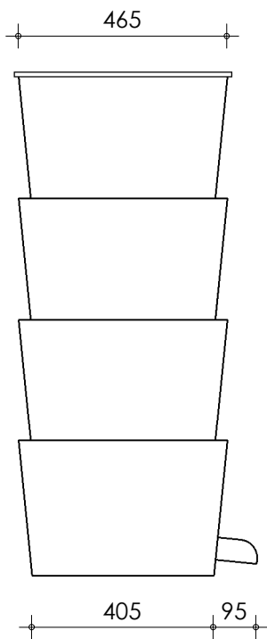
Left-side view
